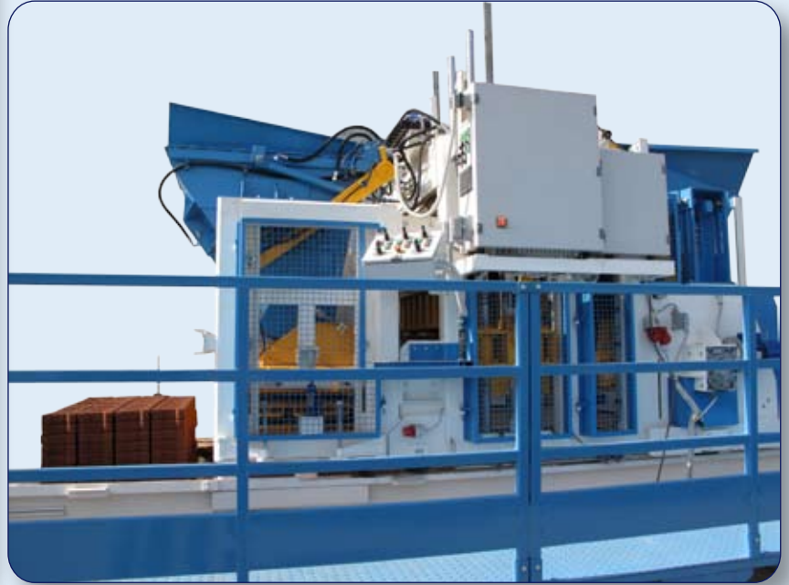
Movable cuber for hollow blocks.
